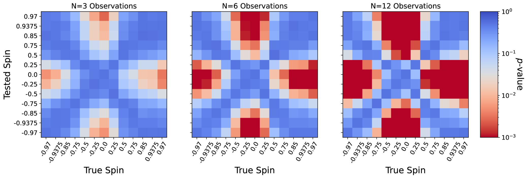
Figure 8. from Vadim Bernshteyn et al 2026 Astrophys. J. 1000 doi:10.3847/1538-4357/ae34af https://dx.doi.org/10.3847/1538-4357/ae34af © 2026. The Author(s). Published by the American Astronomical Society.
