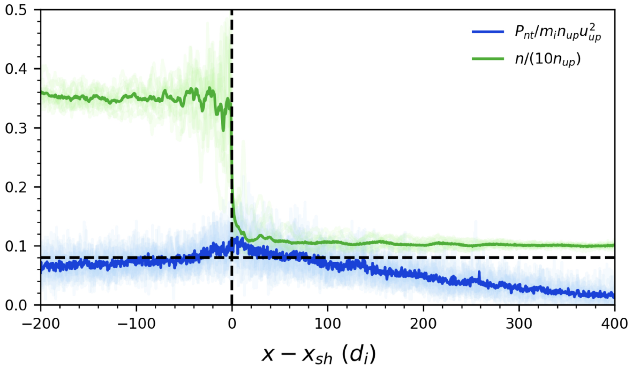
Figure 4. from Colby C. Haggerty et al 2026 Astrophys. J. 998 doi:10.3847/1538-4357/ae2acc https://dx.doi.org/10.3847/1538-4357/ae2acc © 2026. The Author(s). Published by the American Astronomical Society.
