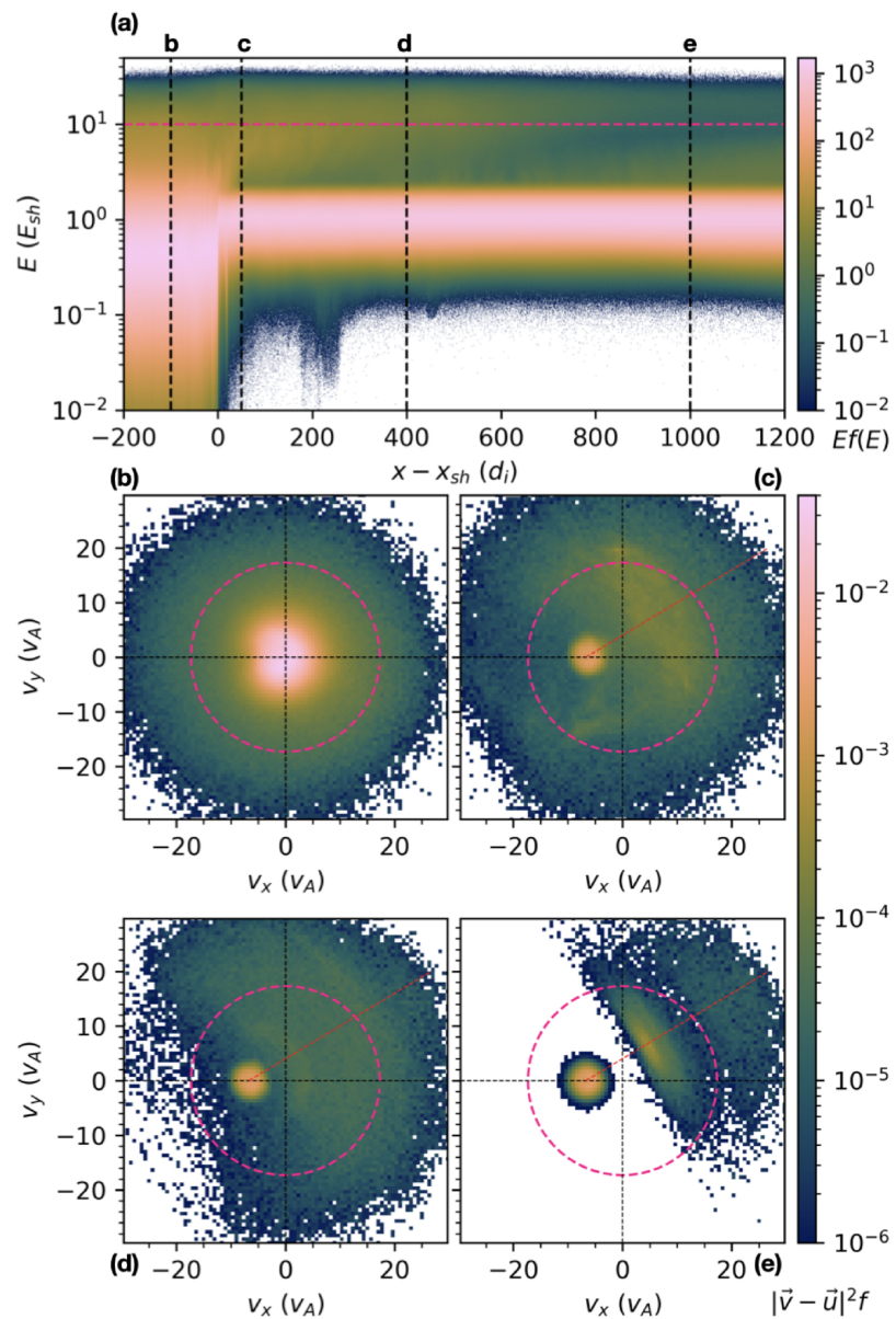
Figure 1. from Colby C. Haggerty et al 2026 Astrophys. J. 998 doi:10.3847/1538-4357/ae2acc https://dx.doi.org/10.3847/1538-4357/ae2acc © 2026. The Author(s). Published by the American Astronomical Society.
