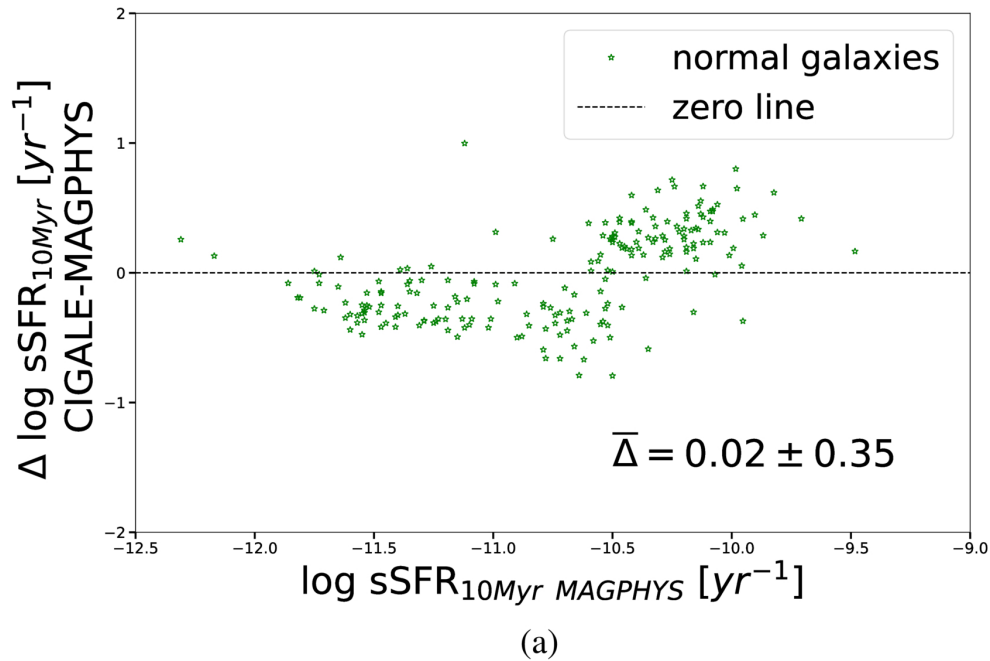
Figure 8. from Maria B. Stone et al 2026 Astrophys. J. 997 doi:10.3847/1538-4357/ae2798 https://dx.doi.org/10.3847/1538-4357/ae2798 © 2026. The Author(s). Published by the American Astronomical Society.
