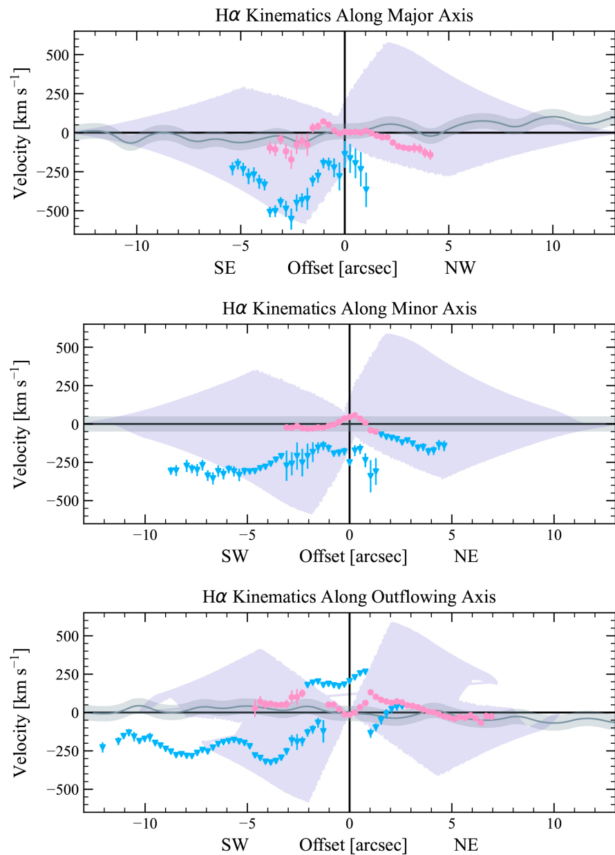
Figure 8. from Maura Kathleen Shea et al 2026 Astrophys. J. 997 doi:10.3847/1538-4357/ae2796 https://dx.doi.org/10.3847/1538-4357/ae2796 © 2026. The Author(s). Published by the American Astronomical Society.
