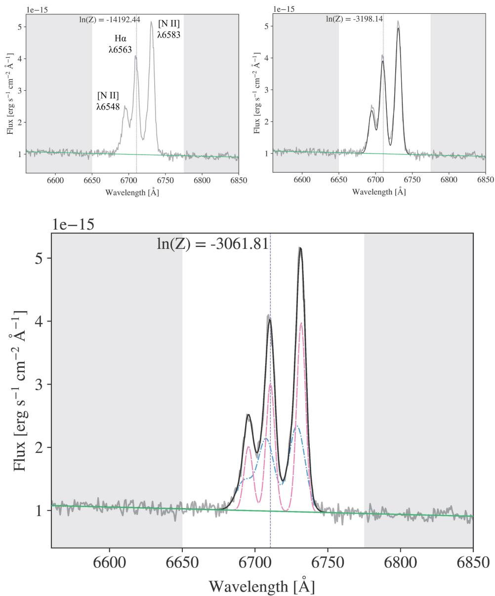
Figure 3. from Maura Kathleen Shea et al 2026 Astrophys. J. 997 doi:10.3847/1538-4357/ae2796 https://dx.doi.org/10.3847/1538-4357/ae2796 © 2026. The Author(s). Published by the American Astronomical Society.
