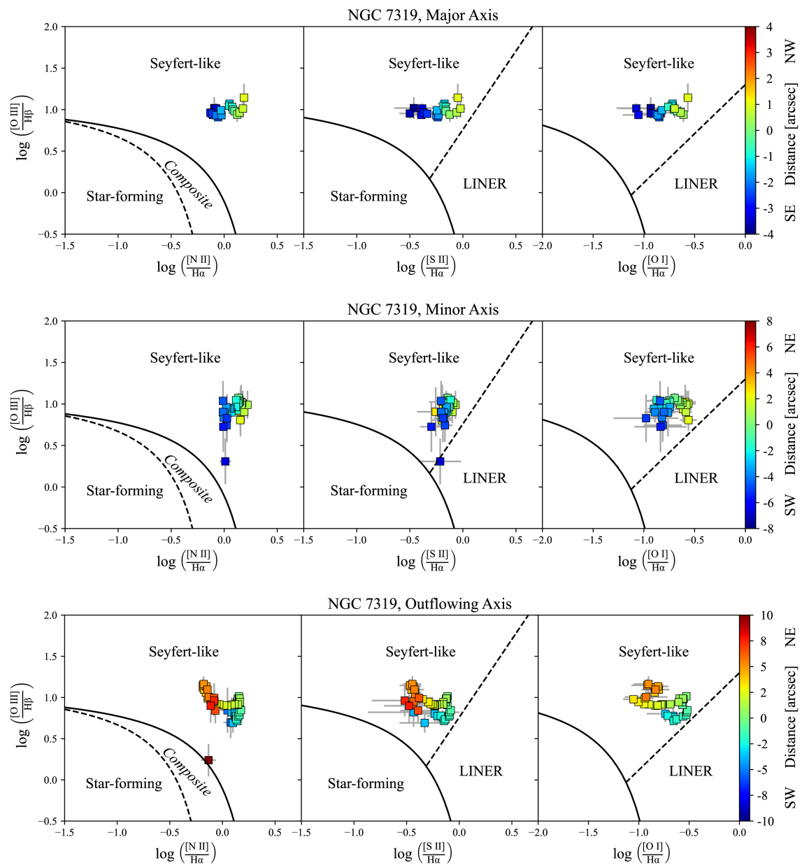
Figure 10. from Maura Kathleen Shea et al 2026 Astrophys. J. 997 doi:10.3847/1538-4357/ae2796 https://dx.doi.org/10.3847/1538-4357/ae2796 © 2026. The Author(s). Published by the American Astronomical Society.
