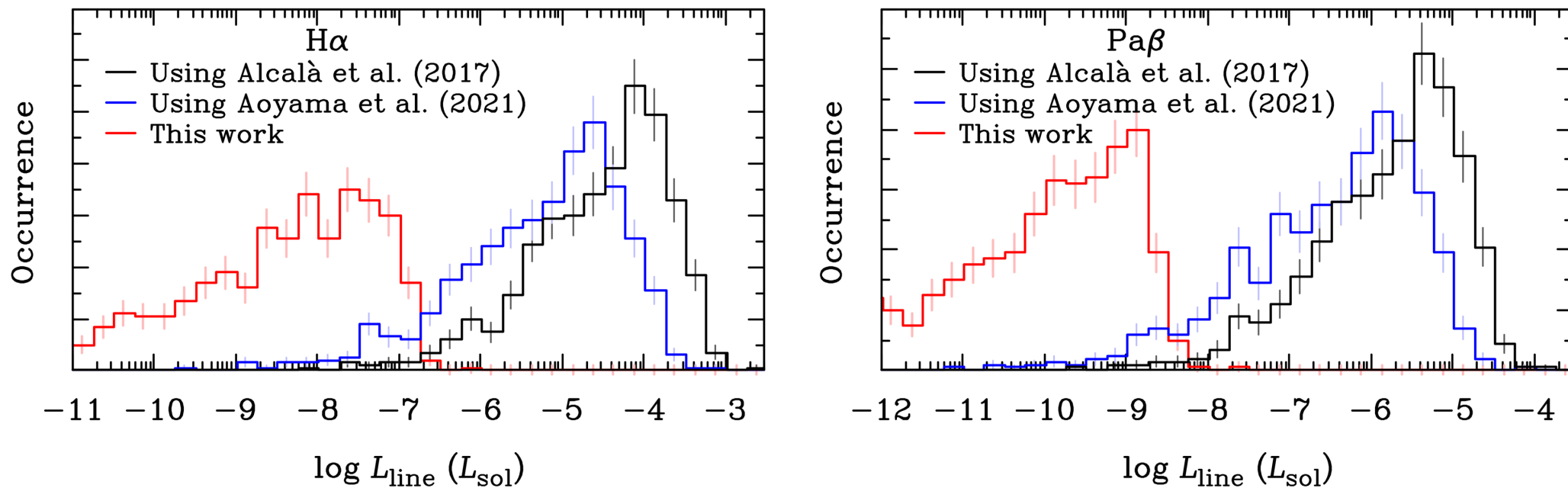
Figure 7. from Gabriel-Dominique Marleau 2026 Astrophys. J. 1000 doi:10.3847/1538-4357/ae2604 https://dx.doi.org/10.3847/1538-4357/ae2604 © 2026. The Author(s). Published by the American Astronomical Society.
