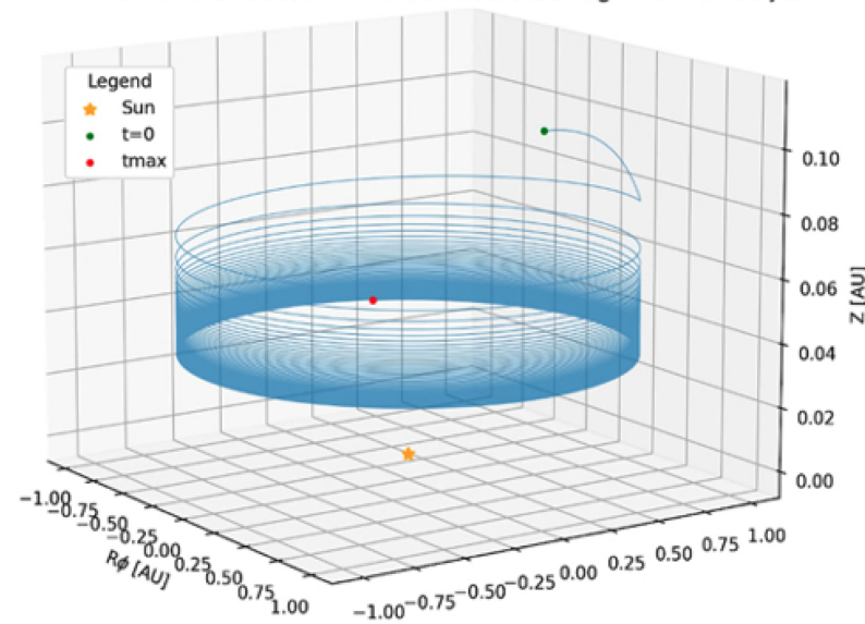
0.1 cm CAI at initial radius of 1.0 AU in disk with scale height 4.6 H for 50.0 years
