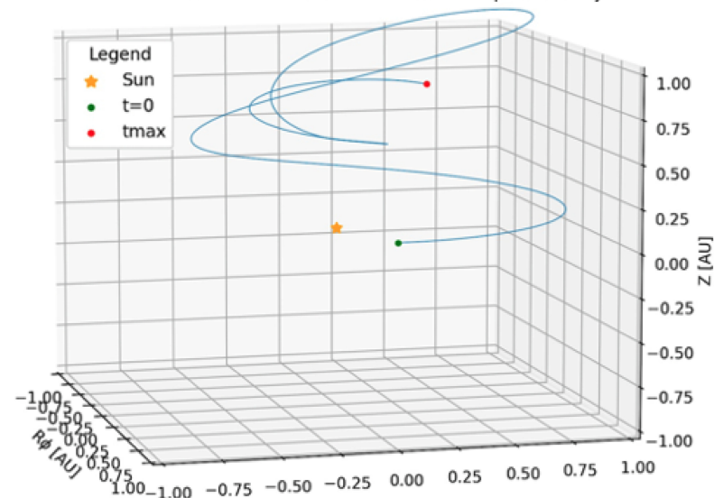
0.0001 cm CAI at initial radius of 1.0 AU in disk near midplane for 2.0 years
