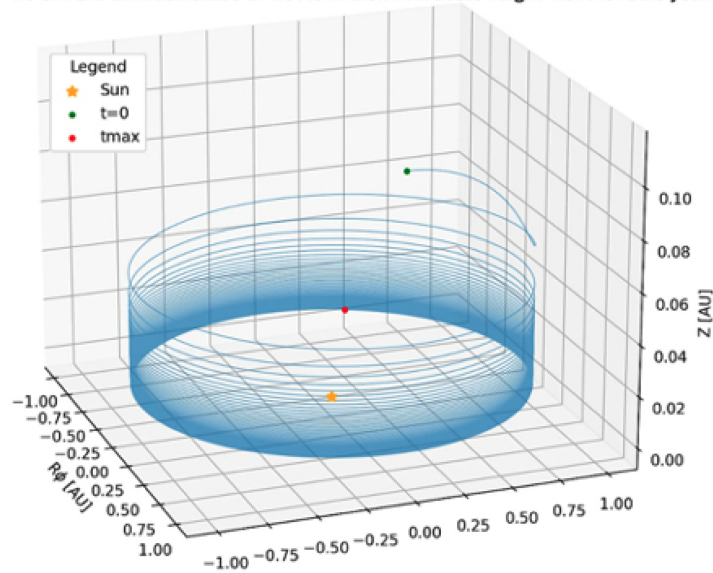
1.0 cm CAI at initial radius of 1.0 AU in disk with scale height 4.6 H for 50.0 years
