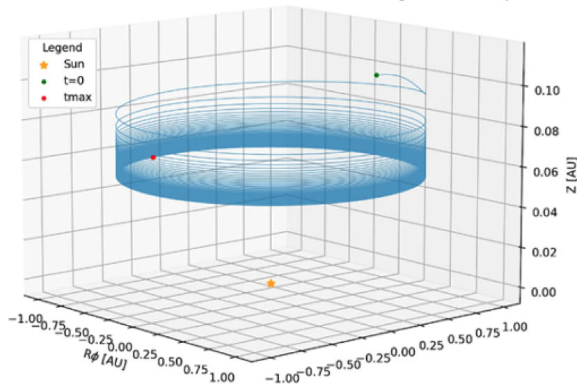
0.01 cm CAI at initial radius of 1.0 AU in disk with scale height 4.6 H for 50.0 years
