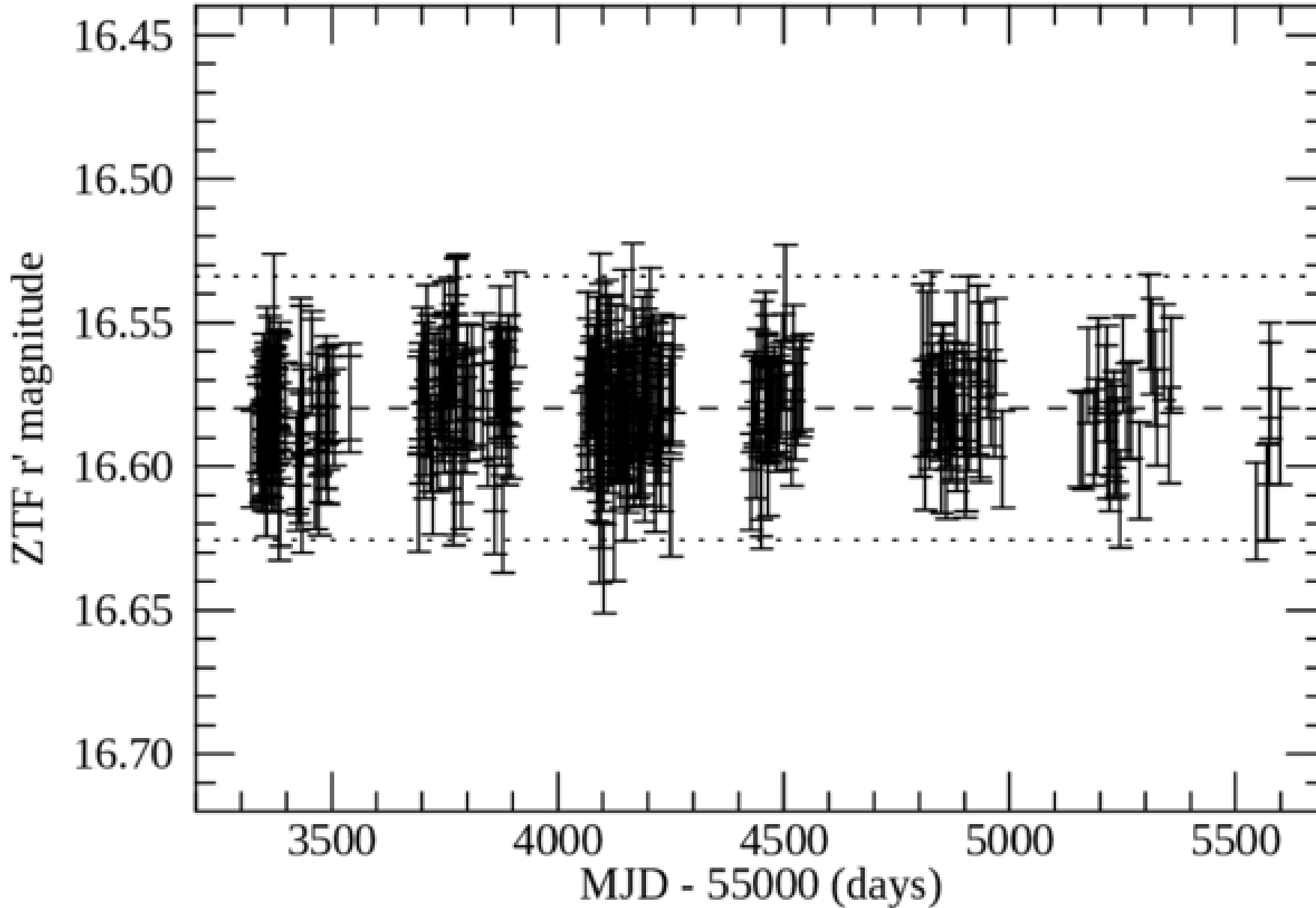
Figure 3. from B. Zuckerman et al 2026 Astrophys. J. 1004 doi:10.3847/1538-4357/ae23c4 https://dx.doi.org/10.3847/1538-4357/ae23c4 © 2026. The Author(s). Published by the American Astronomical Society.
