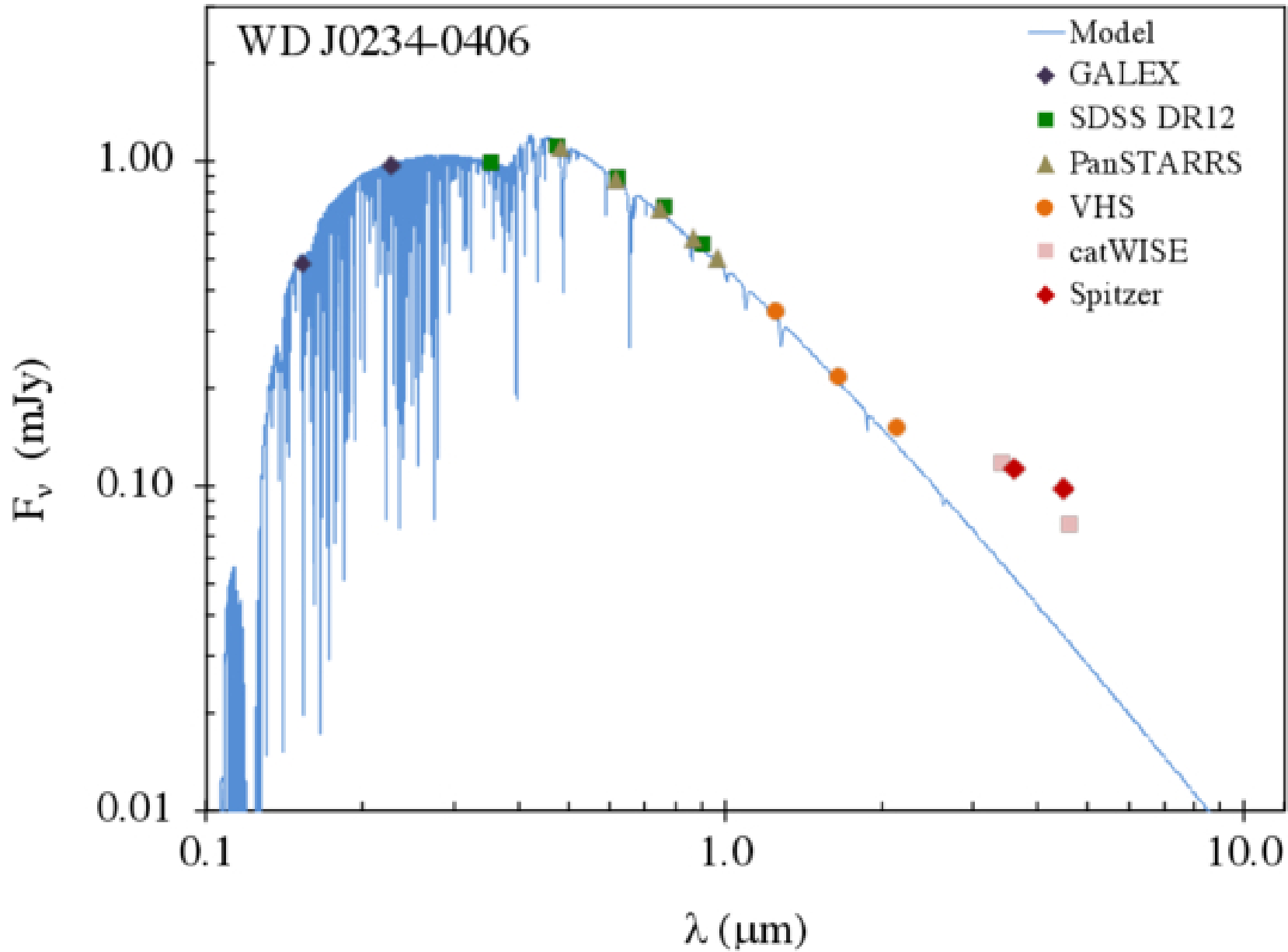
Figure 2. from B. Zuckerman et al 2026 Astrophys. J. 1004 doi:10.3847/1538-4357/ae23c4 https://dx.doi.org/10.3847/1538-4357/ae23c4 © 2026. The Author(s). Published by the American Astronomical Society.
