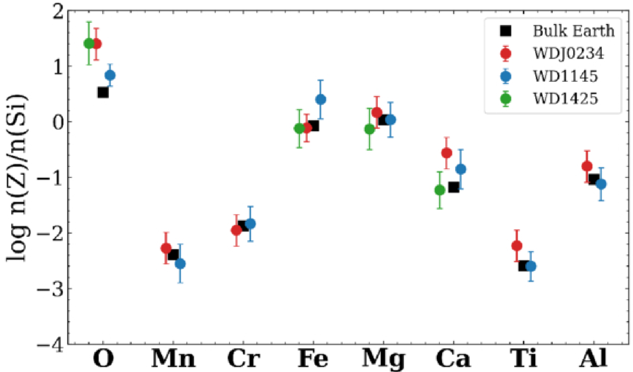
Figure 14. from B. Zuckerman et al 2026 Astrophys. J. 1004 doi:10.3847/1538-4357/ae23c4 https://dx.doi.org/10.3847/1538-4357/ae23c4 © 2026. The Author(s). Published by the American Astronomical Society.
