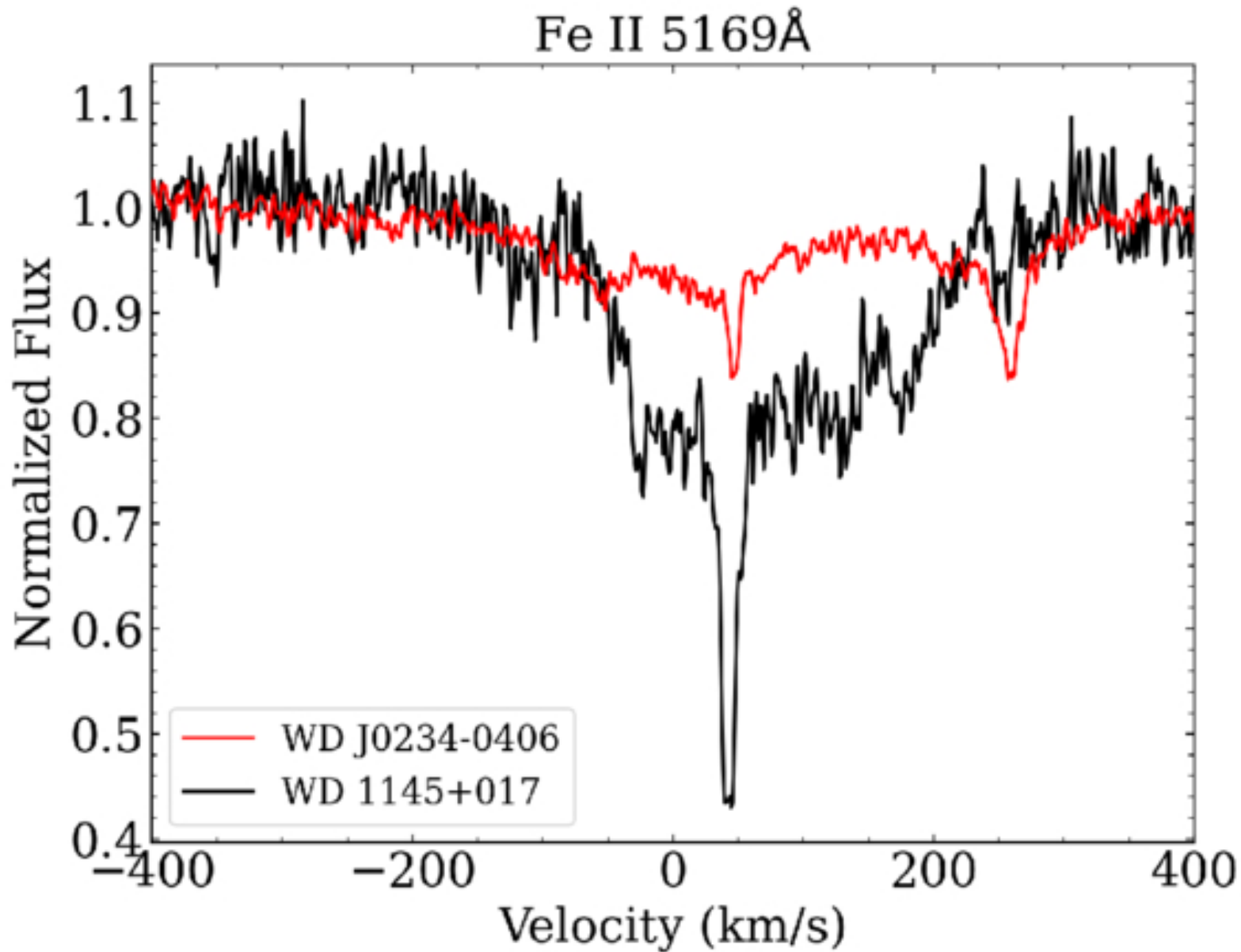
Figure 13. from B. Zuckerman et al 2026 Astrophys. J. 1004 doi:10.3847/1538-4357/ae23c4 https://dx.doi.org/10.3847/1538-4357/ae23c4 © 2026. The Author(s). Published by the American Astronomical Society.
