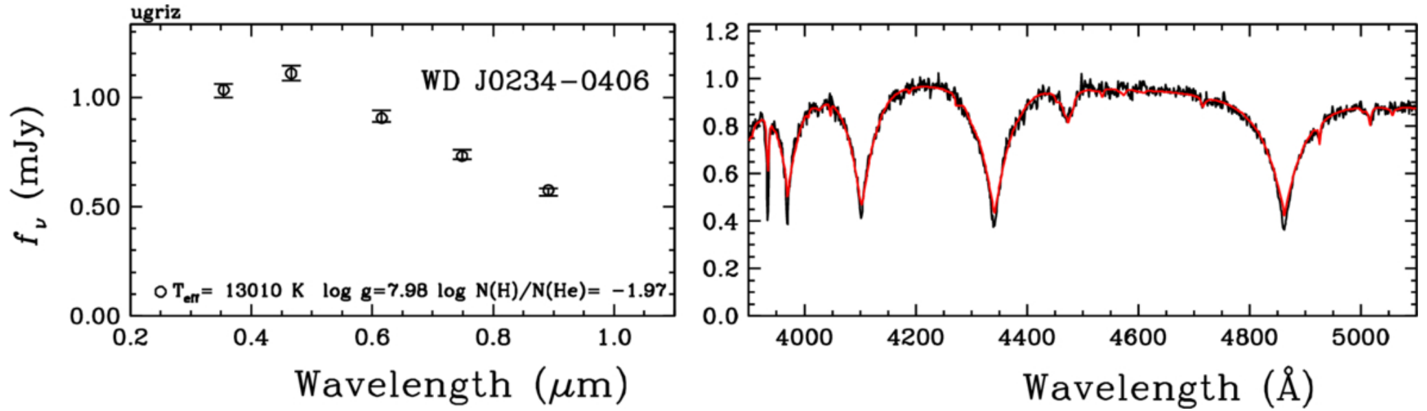
Figure 1. from B. Zuckerman et al 2026 Astrophys. J. 1004 doi:10.3847/1538-4357/ae23c4 https://dx.doi.org/10.3847/1538-4357/ae23c4 © 2026. The Author(s). Published by the American Astronomical Society.
