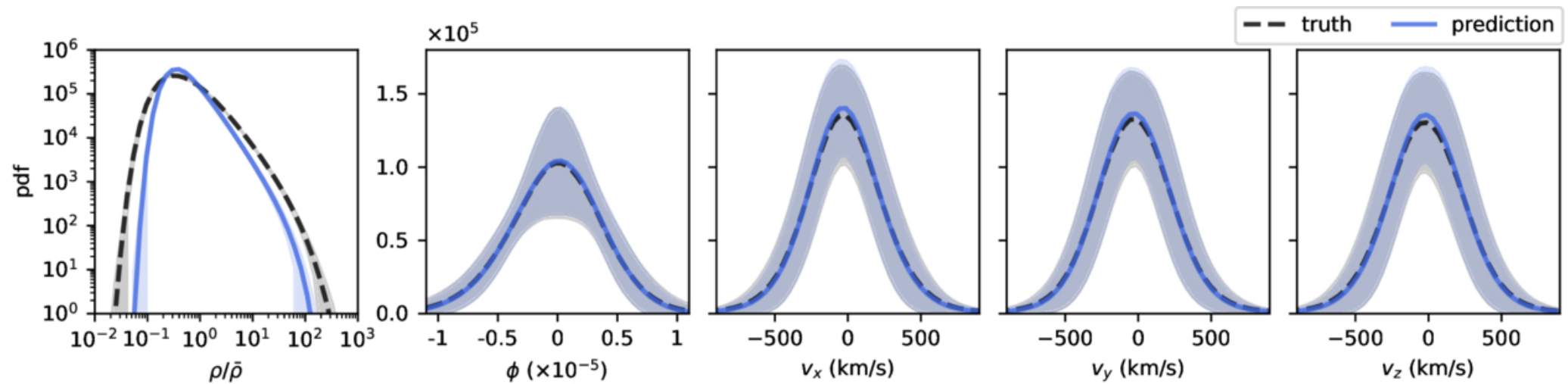
Figure 8. from Alexandra Dupuy et al 2026 Astrophys. J. 997 doi:10.3847/1538-4357/ae21d0 https://dx.doi.org/10.3847/1538-4357/ae21d0 © 2026. The Author(s). Published by the American Astronomical Society.
