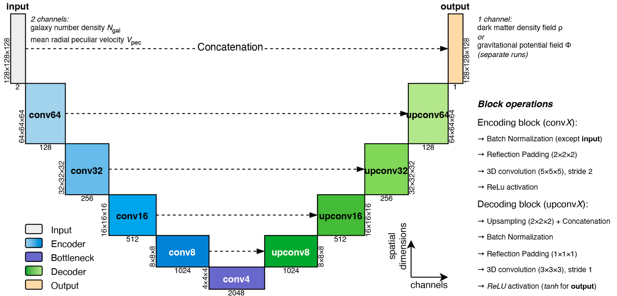
Figure 4. from Alexandra Dupuy et al 2026 Astrophys. J. 997 doi:10.3847/1538-4357/ae21d0 https://dx.doi.org/10.3847/1538-4357/ae21d0 © 2026. The Author(s). Published by the American Astronomical Society.
