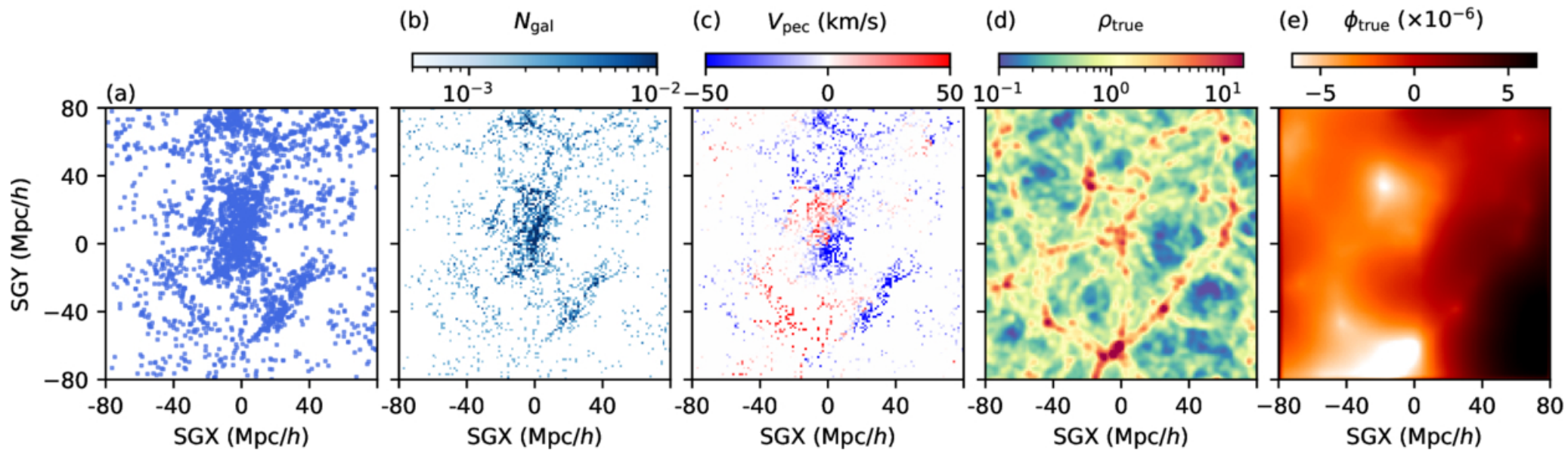
Figure 2. from Alexandra Dupuy et al 2026 Astrophys. J. 997 doi:10.3847/1538-4357/ae21d0 https://dx.doi.org/10.3847/1538-4357/ae21d0 © 2026. The Author(s). Published by the American Astronomical Society.
