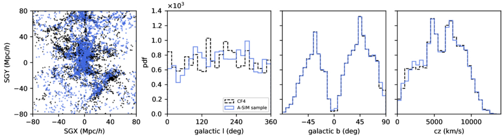
Figure 1. from Alexandra Dupuy et al 2026 Astrophys. J. 997 doi:10.3847/1538-4357/ae21d0 https://dx.doi.org/10.3847/1538-4357/ae21d0 © 2026. The Author(s). Published by the American Astronomical Society.
