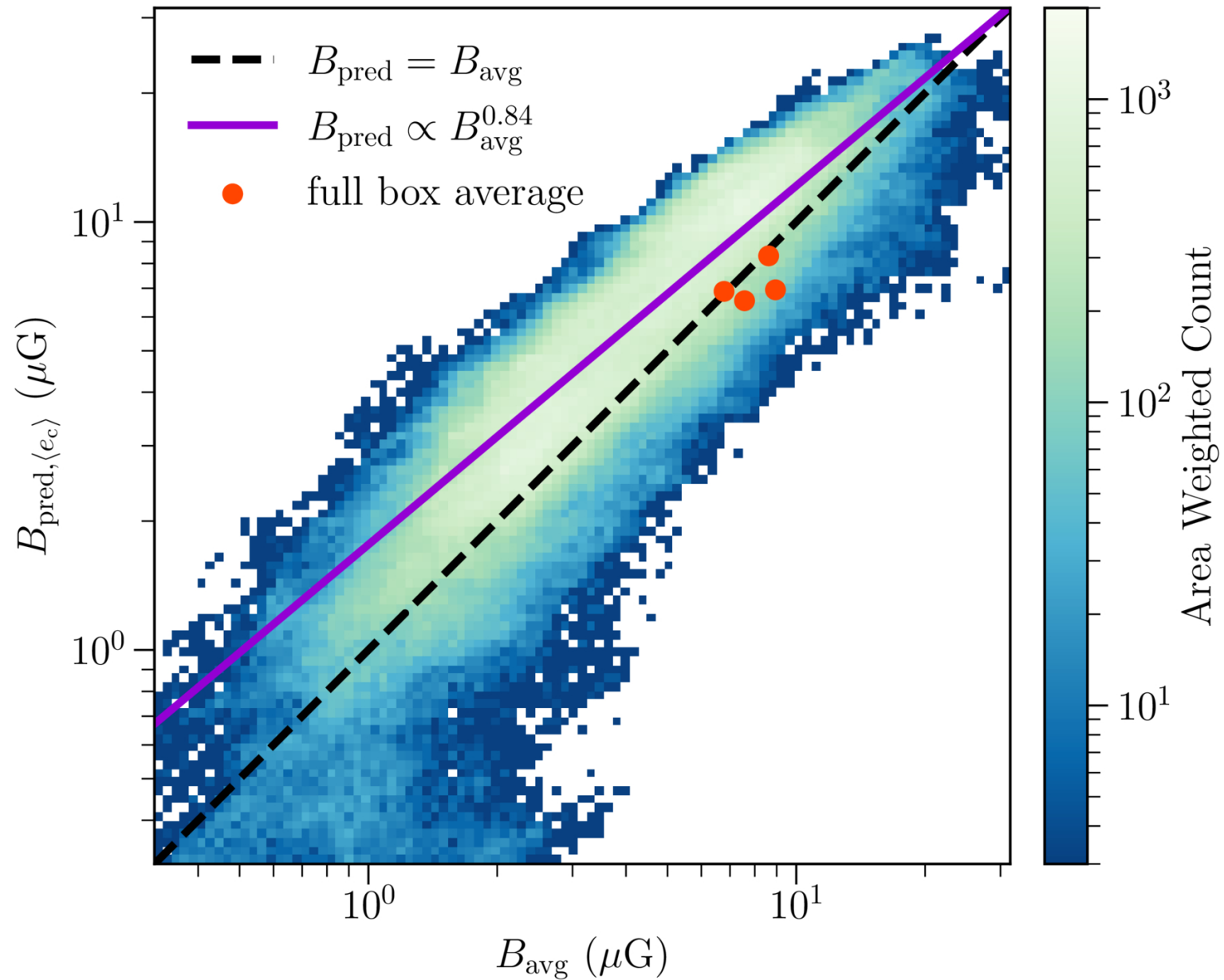
Figure 8. from Nora B. Linzer et al 2026 Astrophys. J. 996 doi:10.3847/1538-4357/ae2019 https://dx.doi.org/10.3847/1538-4357/ae2019 © 2025. The Author(s). Published by the American Astronomical Society.
