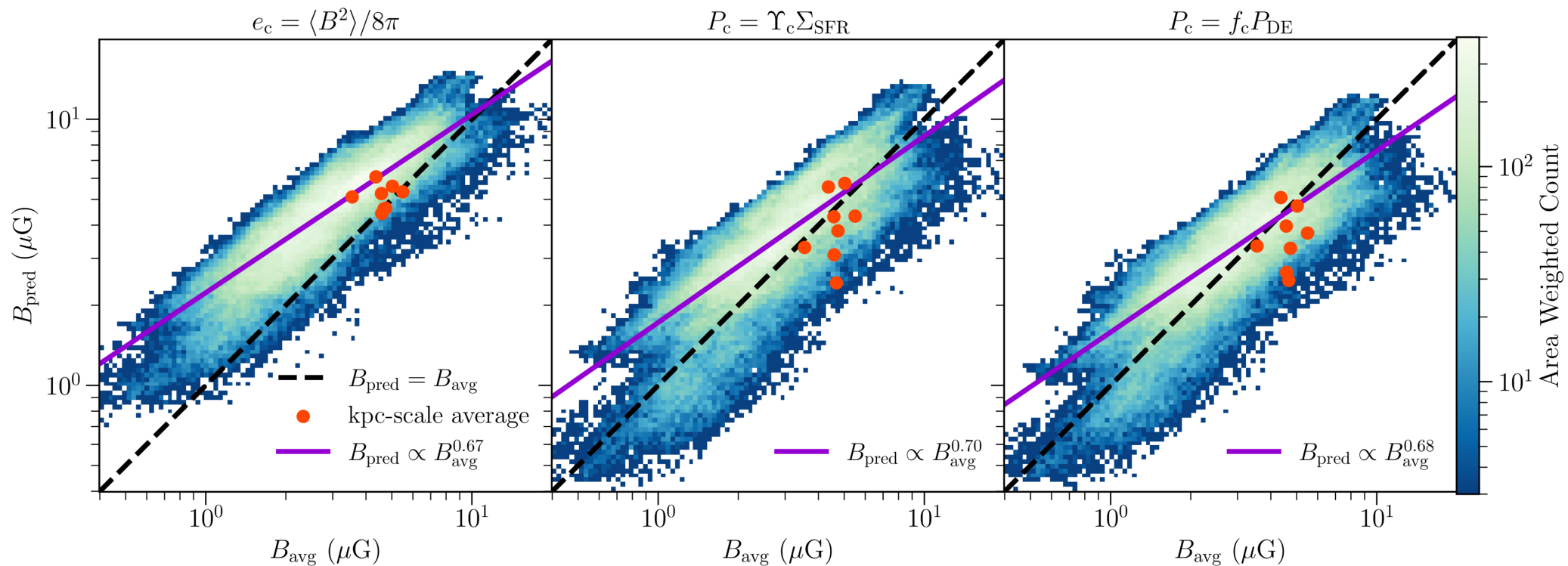
Figure 7. from Nora B. Linzer et al 2026 Astrophys. J. 996 doi:10.3847/1538-4357/ae2019 https://dx.doi.org/10.3847/1538-4357/ae2019 © 2025. The Author(s). Published by the American Astronomical Society.
