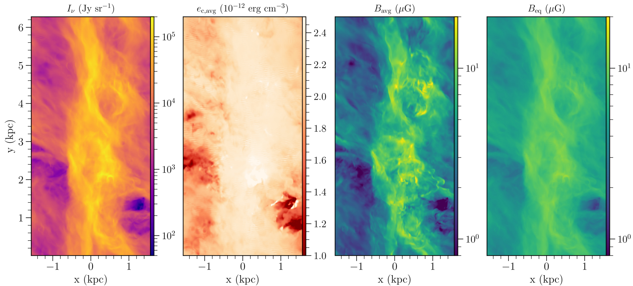
Figure 4. from Nora B. Linzer et al 2026 Astrophys. J. 996 doi:10.3847/1538-4357/ae2019 https://dx.doi.org/10.3847/1538-4357/ae2019 © 2025. The Author(s). Published by the American Astronomical Society.
