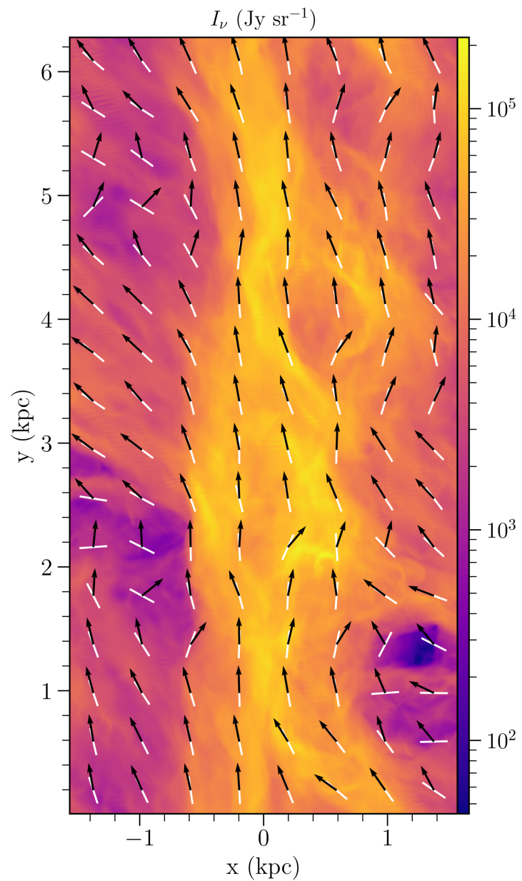
Figure 10. from Nora B. Linzer et al 2026 Astrophys. J. 996 doi:10.3847/1538-4357/ae2019 https://dx.doi.org/10.3847/1538-4357/ae2019 © 2025. The Author(s). Published by the American Astronomical Society.
