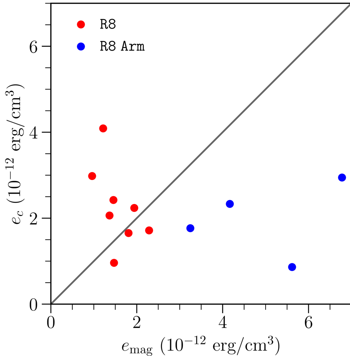
Figure 1. from Nora B. Linzer et al 2026 Astrophys. J. 996 doi:10.3847/1538-4357/ae2019 https://dx.doi.org/10.3847/1538-4357/ae2019 © 2025. The Author(s). Published by the American Astronomical Society.
