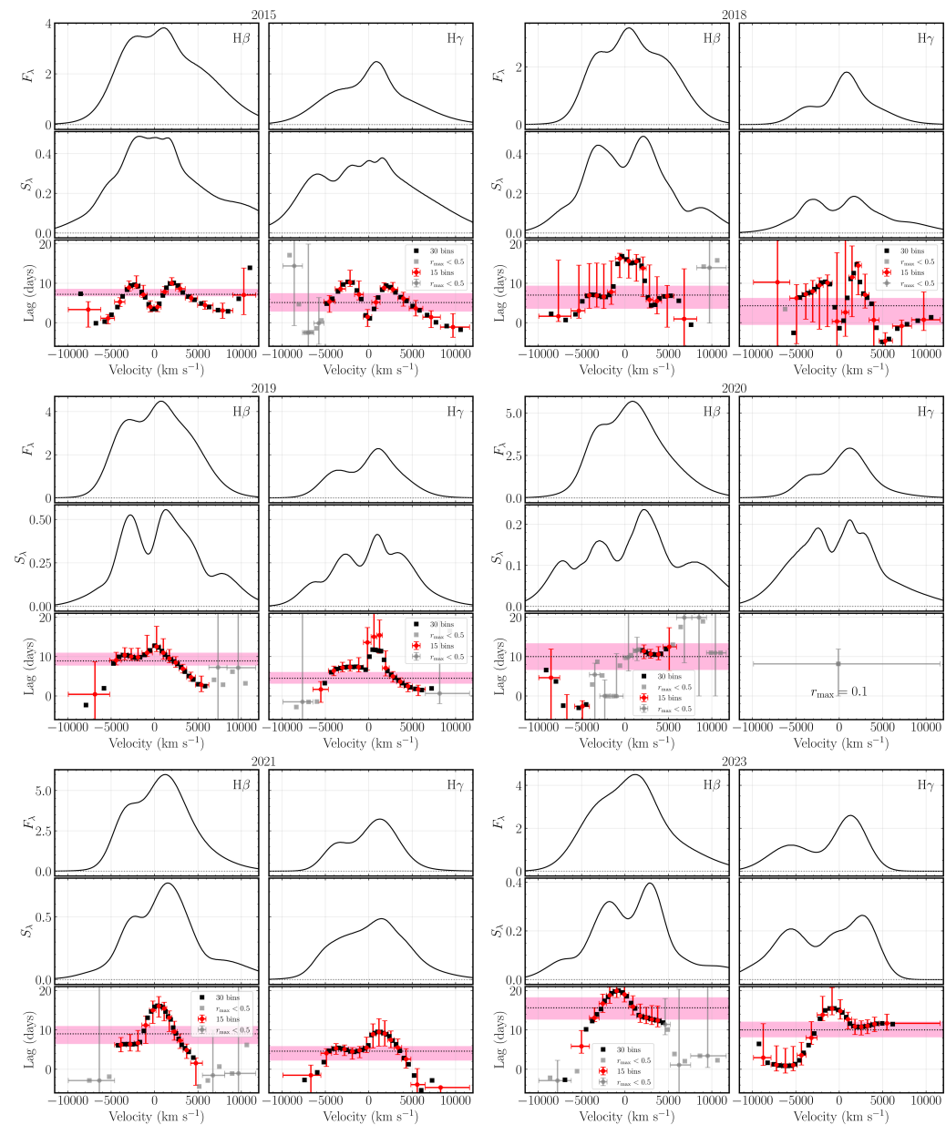
Figure 4. from Wen-Zhe Xi et al 2025 Astrophys. J. 995 doi:10.3847/1538-4357/ae1ccb https://dx.doi.org/10.3847/1538-4357/ae1ccb © 2025. The Author(s). Published by the American Astronomical Society.
