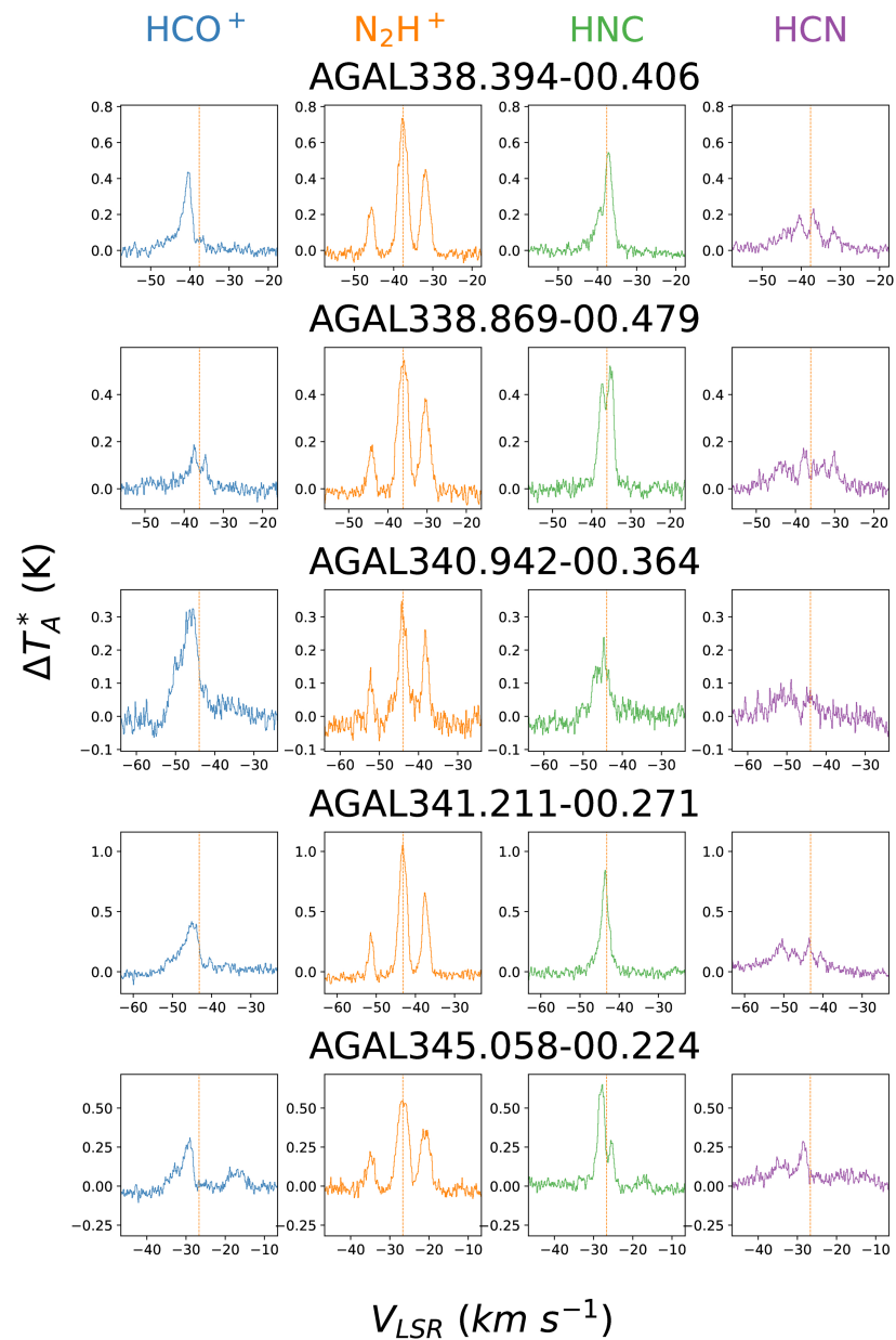
Figure 8. from James M. Jackson et al 2026 Astrophys. J. 998 doi:10.3847/1538-4357/ae19eb https://dx.doi.org/10.3847/1538-4357/ae19eb © 2026. The Author(s). Published by the American Astronomical Society.
