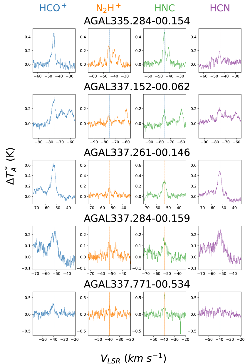
Figure 6. from James M. Jackson et al 2026 Astrophys. J. 998 doi:10.3847/1538-4357/ae19eb https://dx.doi.org/10.3847/1538-4357/ae19eb © 2026. The Author(s). Published by the American Astronomical Society.
