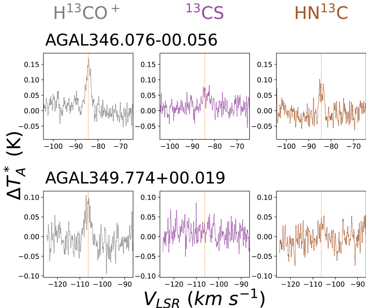
Figure 21. from James M. Jackson et al 2026 Astrophys. J. 998 doi:10.3847/1538-4357/ae19eb https://dx.doi.org/10.3847/1538-4357/ae19eb © 2026. The Author(s). Published by the American Astronomical Society.
