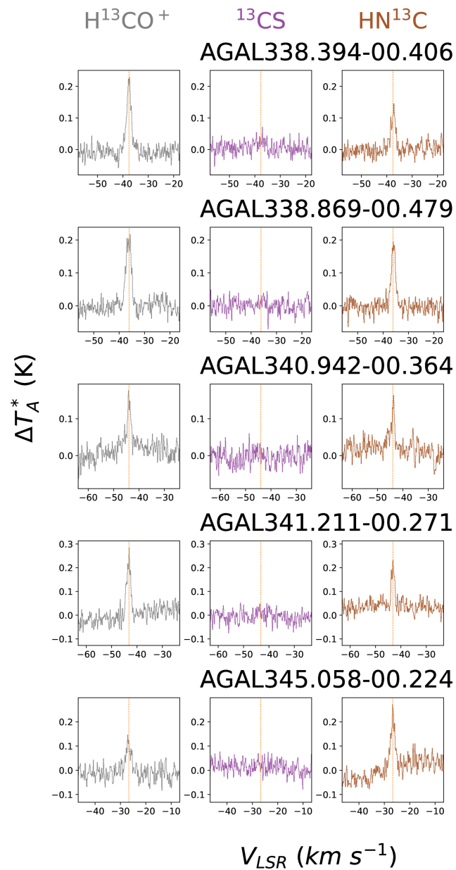
Figure 20. from James M. Jackson et al 2026 Astrophys. J. 998 doi:10.3847/1538-4357/ae19eb https://dx.doi.org/10.3847/1538-4357/ae19eb © 2026. The Author(s). Published by the American Astronomical Society.
