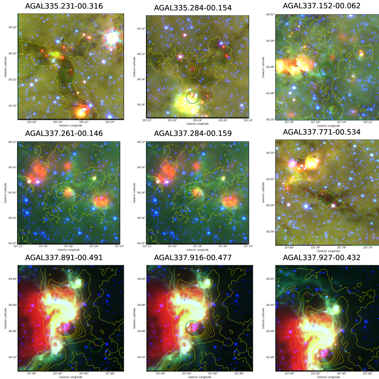
Figure 2. from James M. Jackson et al 2026 Astrophys. J. 998 doi:10.3847/1538-4357/ae19eb https://dx.doi.org/10.3847/1538-4357/ae19eb © 2026. The Author(s). Published by the American Astronomical Society.
