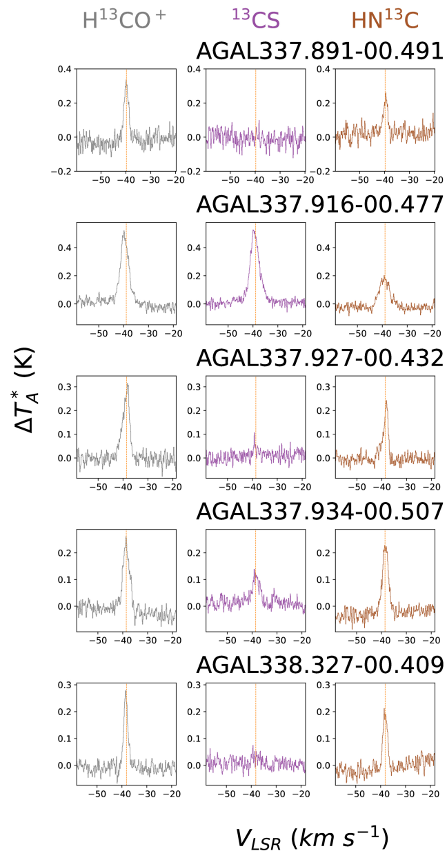
Figure 19. from James M. Jackson et al 2026 Astrophys. J. 998 doi:10.3847/1538-4357/ae19eb https://dx.doi.org/10.3847/1538-4357/ae19eb © 2026. The Author(s). Published by the American Astronomical Society.
