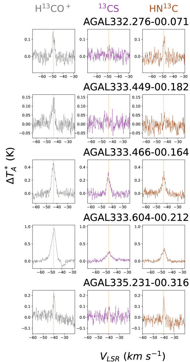
Figure 17. from James M. Jackson et al 2026 Astrophys. J. 998 doi:10.3847/1538-4357/ae19eb https://dx.doi.org/10.3847/1538-4357/ae19eb © 2026. The Author(s). Published by the American Astronomical Society.
