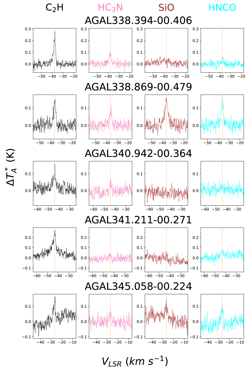
Figure 14. from James M. Jackson et al 2026 Astrophys. J. 998 doi:10.3847/1538-4357/ae19eb https://dx.doi.org/10.3847/1538-4357/ae19eb © 2026. The Author(s). Published by the American Astronomical Society.
