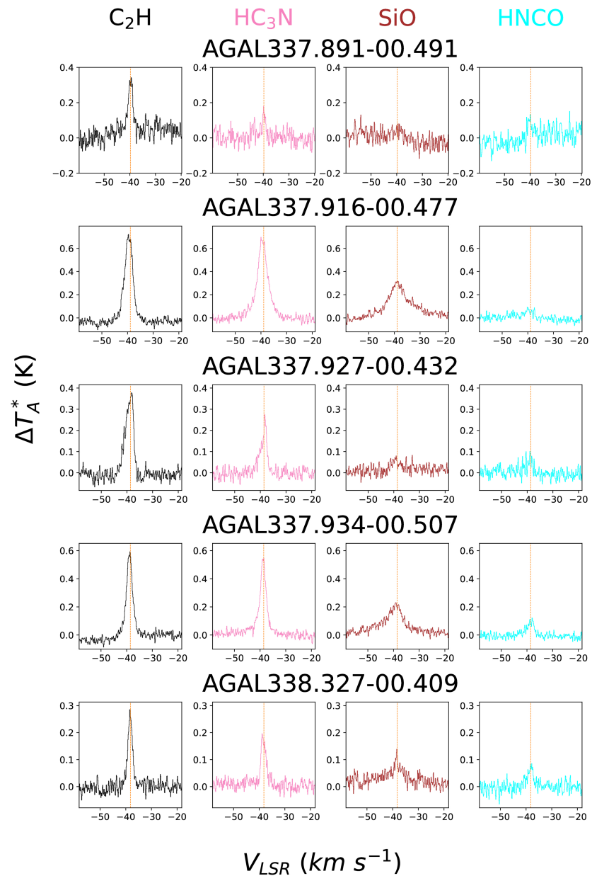
Figure 13. from James M. Jackson et al 2026 Astrophys. J. 998 doi:10.3847/1538-4357/ae19eb https://dx.doi.org/10.3847/1538-4357/ae19eb © 2026. The Author(s). Published by the American Astronomical Society.
