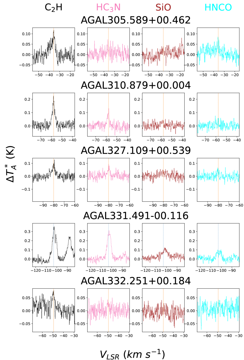
Figure 10. from James M. Jackson et al 2026 Astrophys. J. 998 doi:10.3847/1538-4357/ae19eb https://dx.doi.org/10.3847/1538-4357/ae19eb © 2026. The Author(s). Published by the American Astronomical Society.
