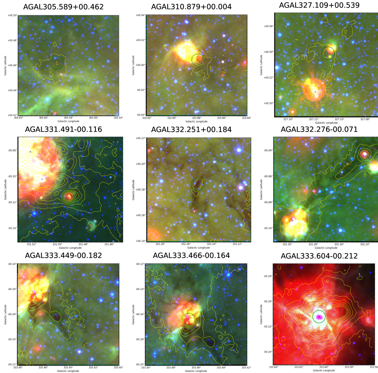
Figure 1. from James M. Jackson et al 2026 Astrophys. J. 998 doi:10.3847/1538-4357/ae19eb https://dx.doi.org/10.3847/1538-4357/ae19eb © 2026. The Author(s). Published by the American Astronomical Society.
