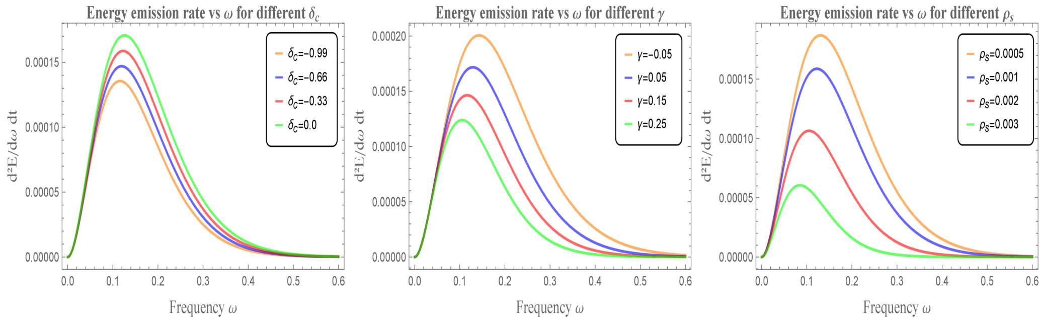
Figure 6. from A. Errehymy et al 2025 Astrophys. J. 995 doi:10.3847/1538-4357/ae197f https://dx.doi.org/10.3847/1538-4357/ae197f © 2025. The Author(s). Published by the American Astronomical Society.
