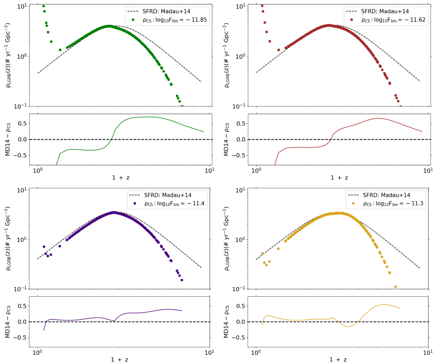
Figure 8. from Dhruv S. Bal et al 2025 Astrophys. J. 994 doi:10.3847/1538-4357/ae1736 https://dx.doi.org/10.3847/1538-4357/ae1736 © 2025. The Author(s). Published by the American Astronomical Society.
