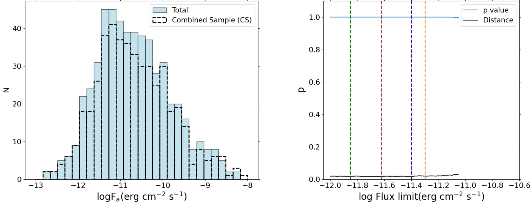
Figure 7. from Dhruv S. Bal et al 2025 Astrophys. J. 994 doi:10.3847/1538-4357/ae1736 https://dx.doi.org/10.3847/1538-4357/ae1736 © 2025. The Author(s). Published by the American Astronomical Society.
