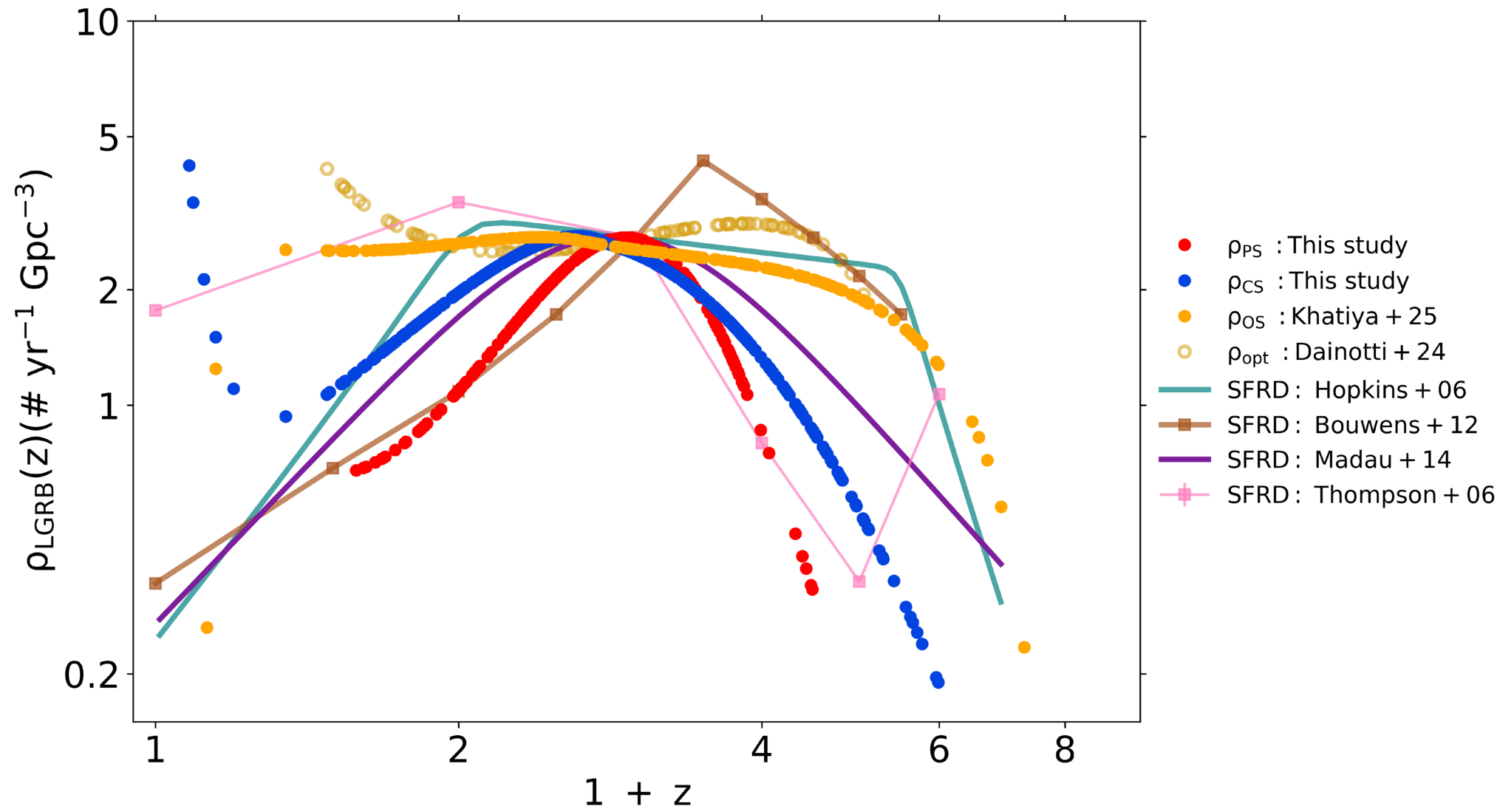
Figure 3. from Dhruv S. Bal et al 2025 Astrophys. J. 994 doi:10.3847/1538-4357/ae1736 https://dx.doi.org/10.3847/1538-4357/ae1736 © 2025. The Author(s). Published by the American Astronomical Society.
