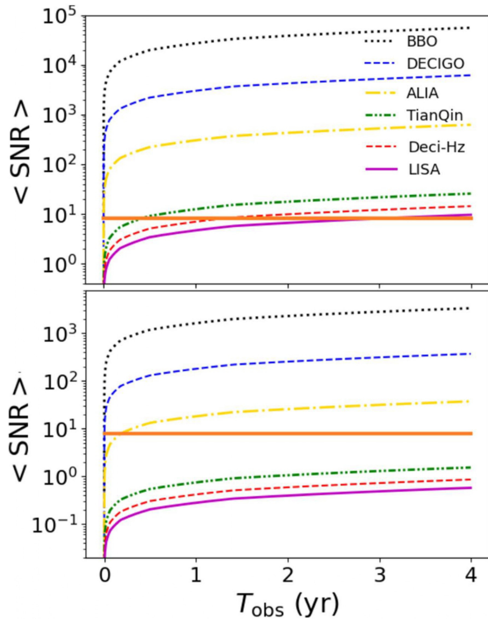
Figure 9. from Mayusree Das et al 2025 Astrophys. J. 995 doi:10.3847/1538-4357/ae1732 https://dx.doi.org/10.3847/1538-4357/ae1732 © 2025. The Author(s). Published by the American Astronomical Society.
