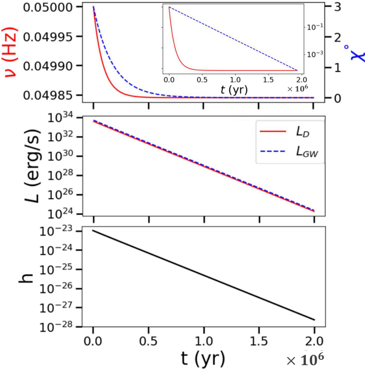
Figure 6. from Mayusree Das et al 2025 Astrophys. J. 995 doi:10.3847/1538-4357/ae1732 https://dx.doi.org/10.3847/1538-4357/ae1732 © 2025. The Author(s). Published by the American Astronomical Society.
