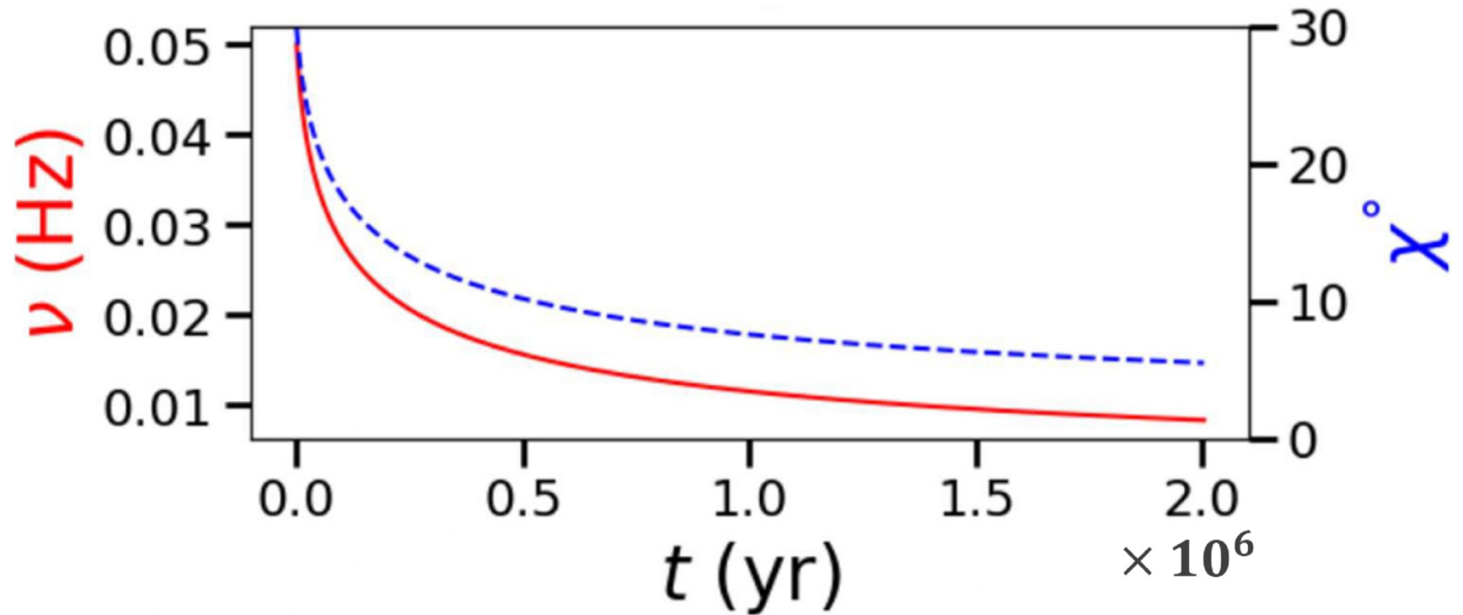
Figure 5. from Mayusree Das et al 2025 Astrophys. J. 995 doi:10.3847/1538-4357/ae1732 https://dx.doi.org/10.3847/1538-4357/ae1732 © 2025. The Author(s). Published by the American Astronomical Society.
