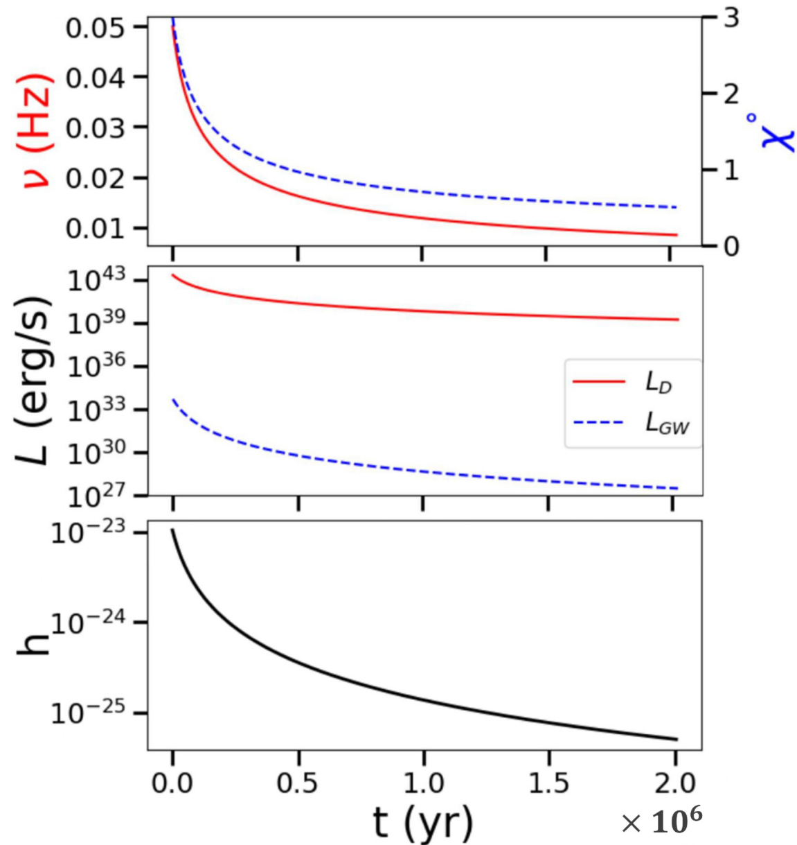
Figure 4. from Mayusree Das et al 2025 Astrophys. J. 995 doi:10.3847/1538-4357/ae1732 https://dx.doi.org/10.3847/1538-4357/ae1732 © 2025. The Author(s). Published by the American Astronomical Society.
