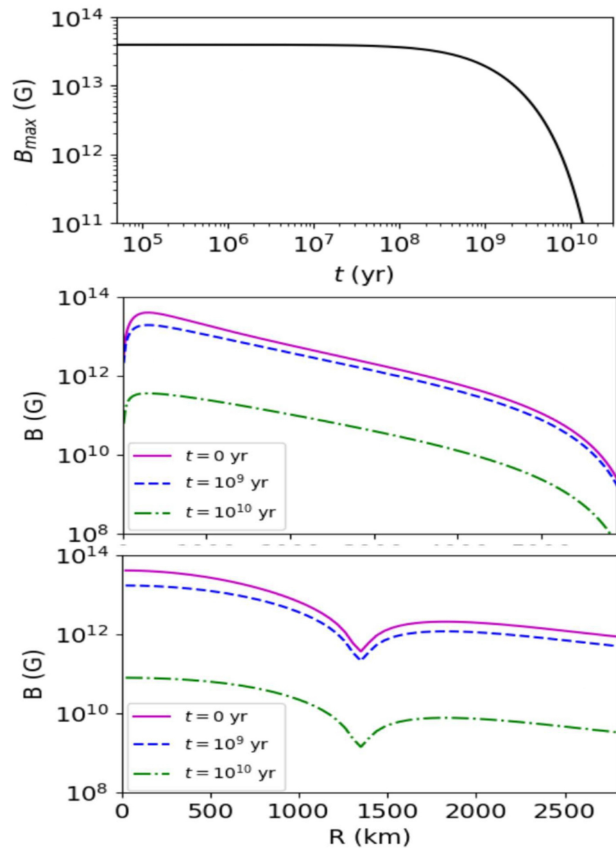
Figure 3. from Mayusree Das et al 2025 Astrophys. J. 995 doi:10.3847/1538-4357/ae1732 https://dx.doi.org/10.3847/1538-4357/ae1732 © 2025. The Author(s). Published by the American Astronomical Society.
