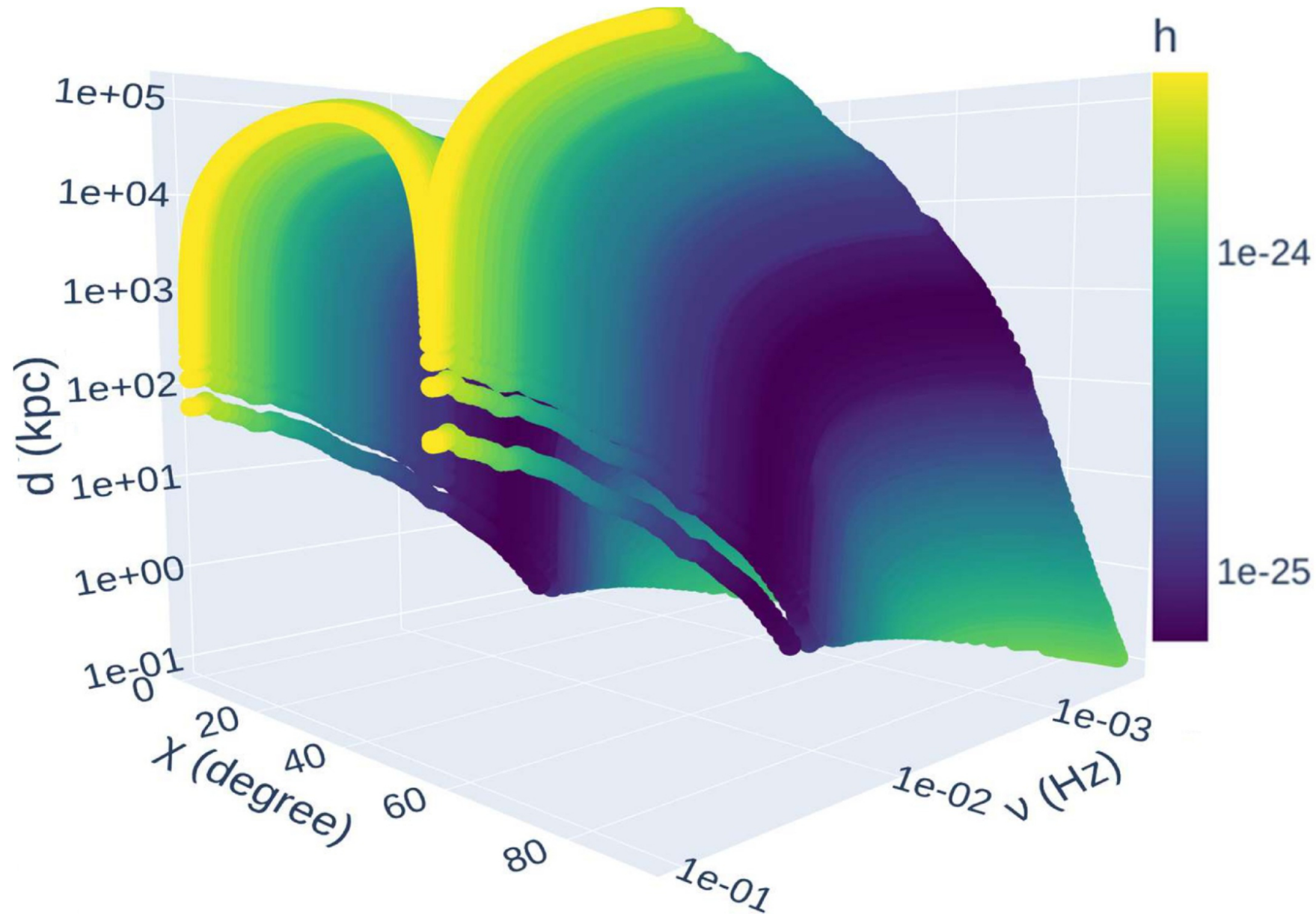
Figure 10. from Mayusree Das et al 2025 Astrophys. J. 995 doi:10.3847/1538-4357/ae1732 https://dx.doi.org/10.3847/1538-4357/ae1732 © 2025. The Author(s). Published by the American Astronomical Society.
