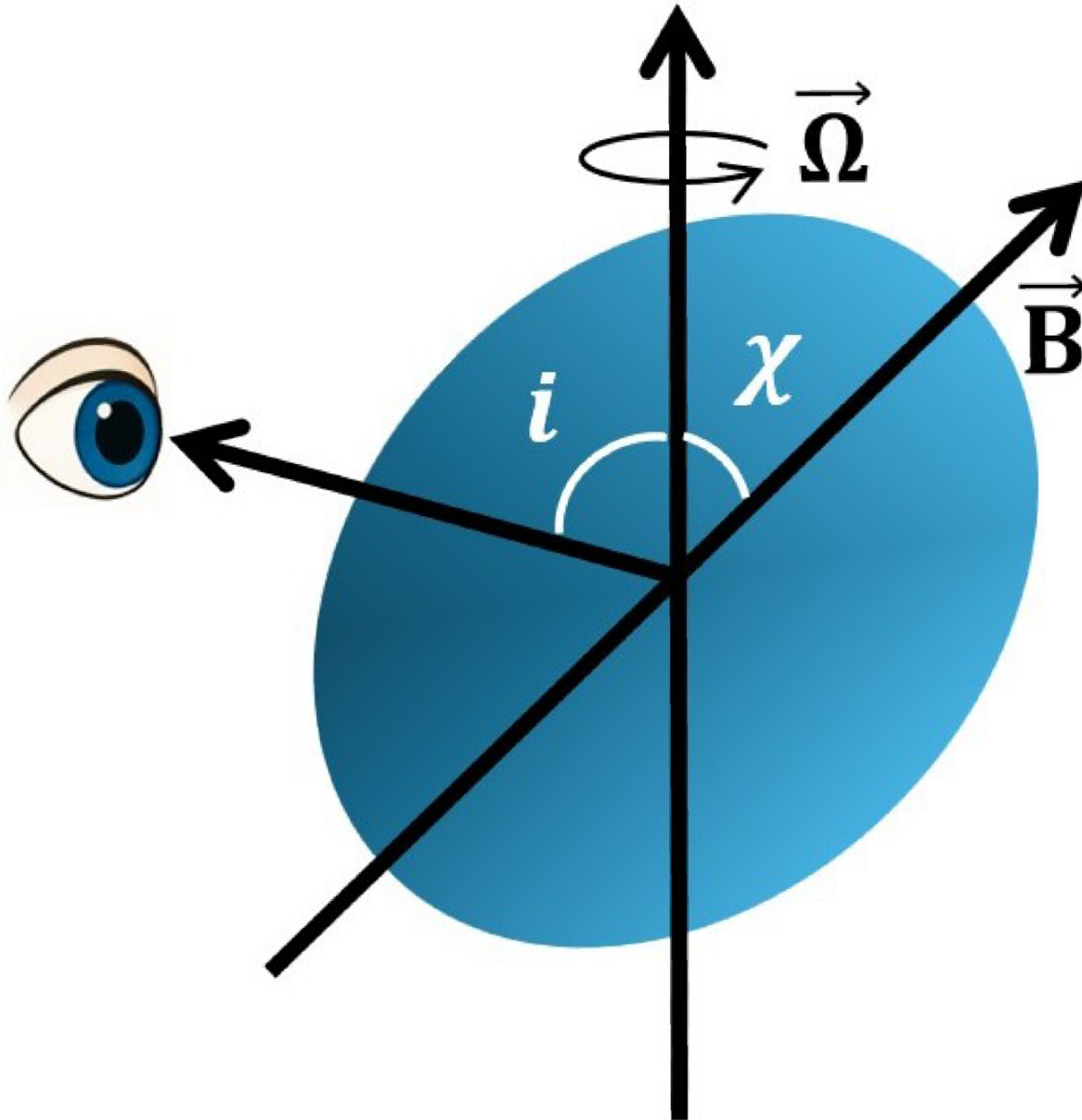
Figure 1. from Mayusree Das et al 2025 Astrophys. J. 995 doi:10.3847/1538-4357/ae1732 https://dx.doi.org/10.3847/1538-4357/ae1732 © 2025. The Author(s). Published by the American Astronomical Society.
