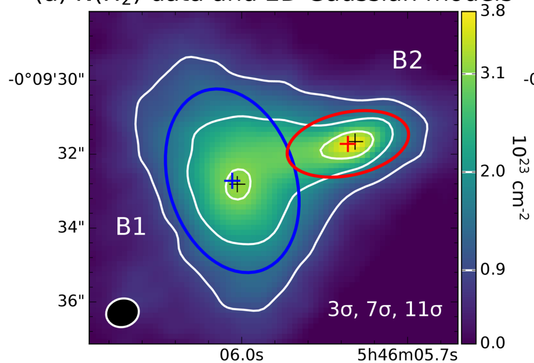
(a) N(\text{H}_2) data and 2D Gaussian models
