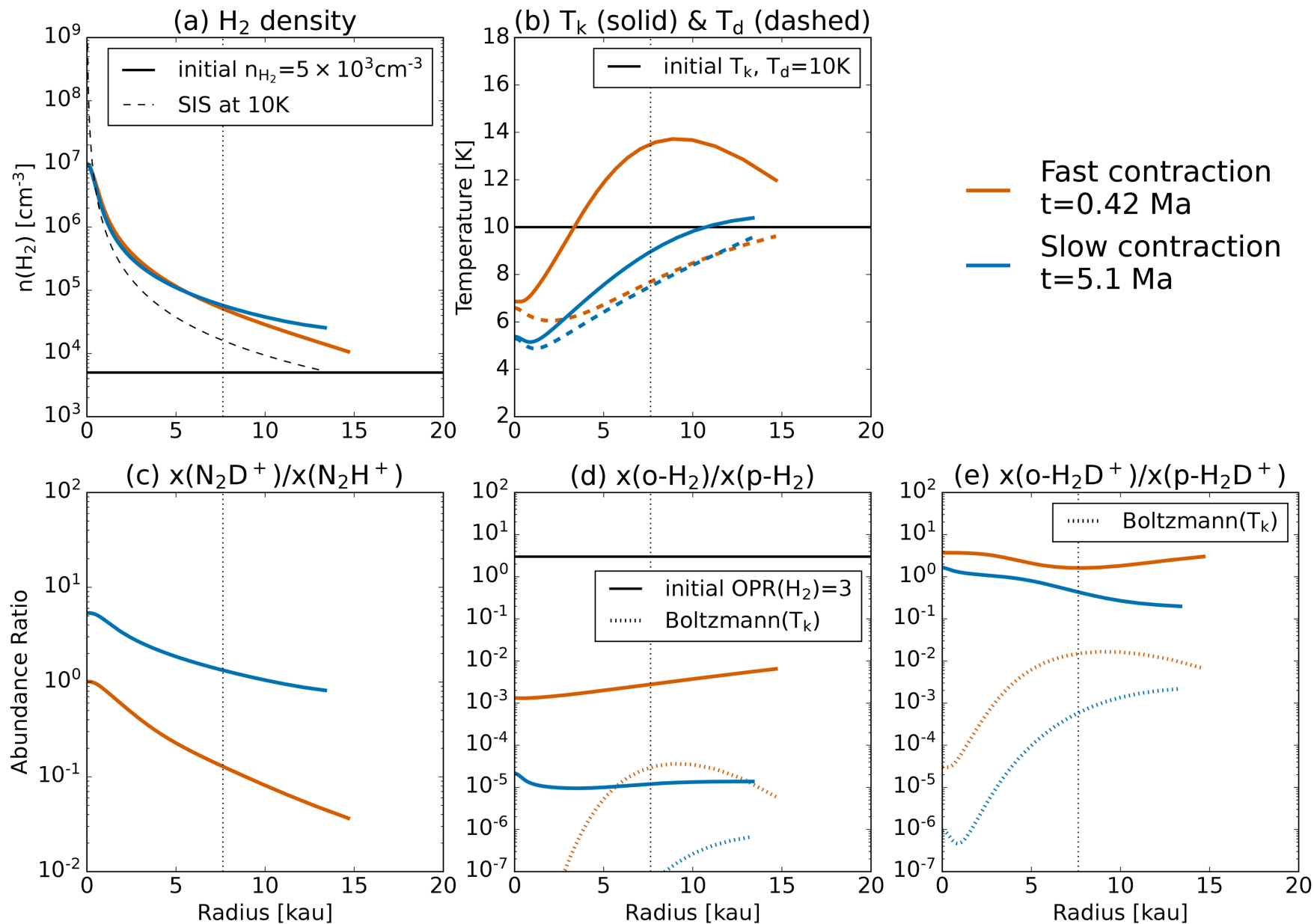
Figure 7. from Sheng-Jun Lin et al 2025 Astrophys. J. 995 doi:10.3847/1538-4357/ae0cb5 https://dx.doi.org/10.3847/1538-4357/ae0cb5 © 2025. The Author(s). Published by the American Astronomical Society.
