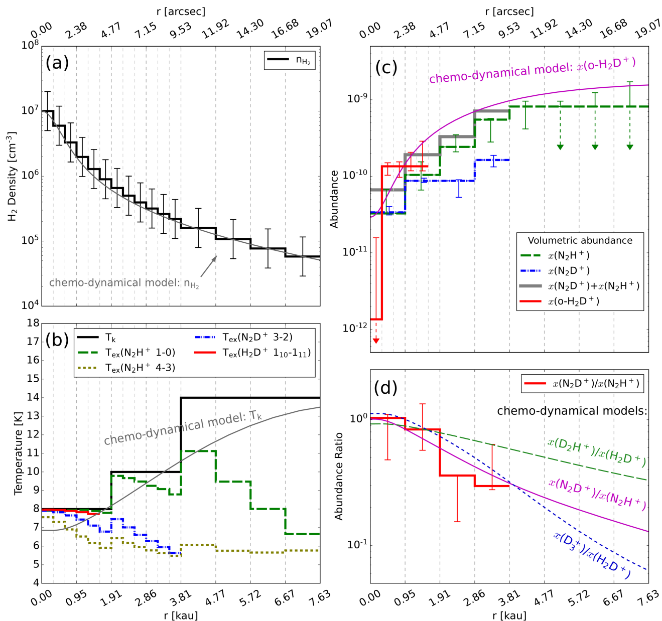
Figure 5. from Sheng-Jun Lin et al 2025 Astrophys. J. 995 doi:10.3847/1538-4357/ae0cb5 https://dx.doi.org/10.3847/1538-4357/ae0cb5 © 2025. The Author(s). Published by the American Astronomical Society.
