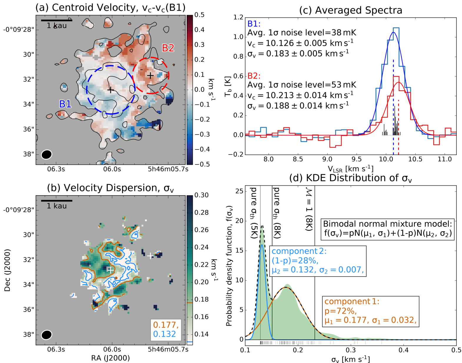
Figure 3. from Sheng-Jun Lin et al 2025 Astrophys. J. 995 doi:10.3847/1538-4357/ae0cb5 https://dx.doi.org/10.3847/1538-4357/ae0cb5 © 2025. The Author(s). Published by the American Astronomical Society.
